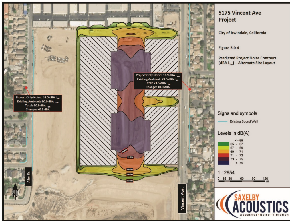
Figure B: Projected Noise Contours for Multi-Building Alternative (DEIR at 5.0-33 Fig. 5.0-4)
