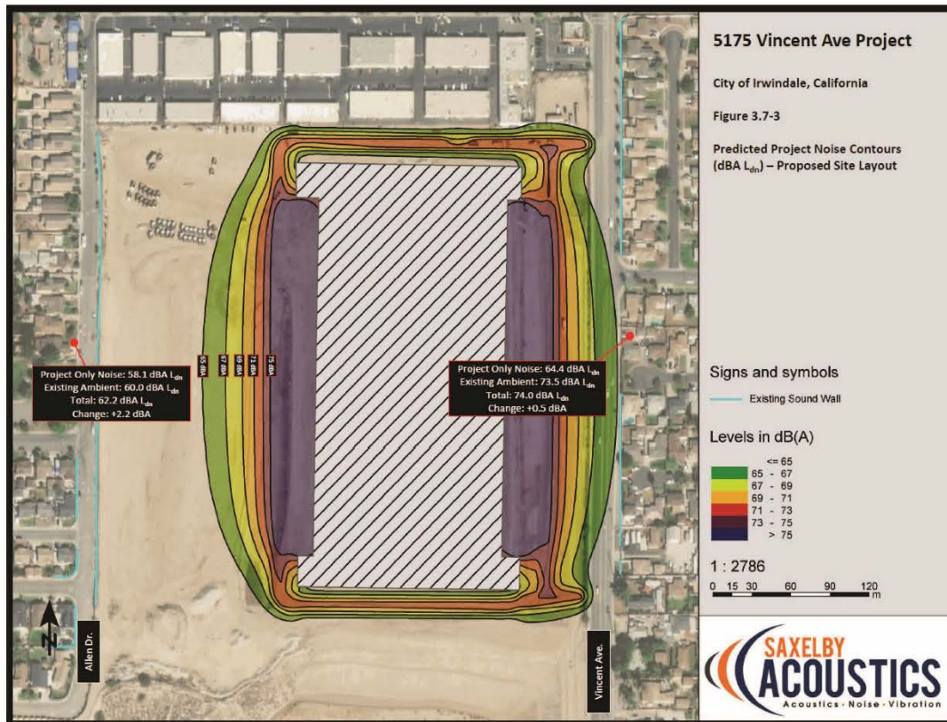
Figure A: Projected Noise Contours for Project (DEIR at 3.7-25 Fig. 3-7.3)
